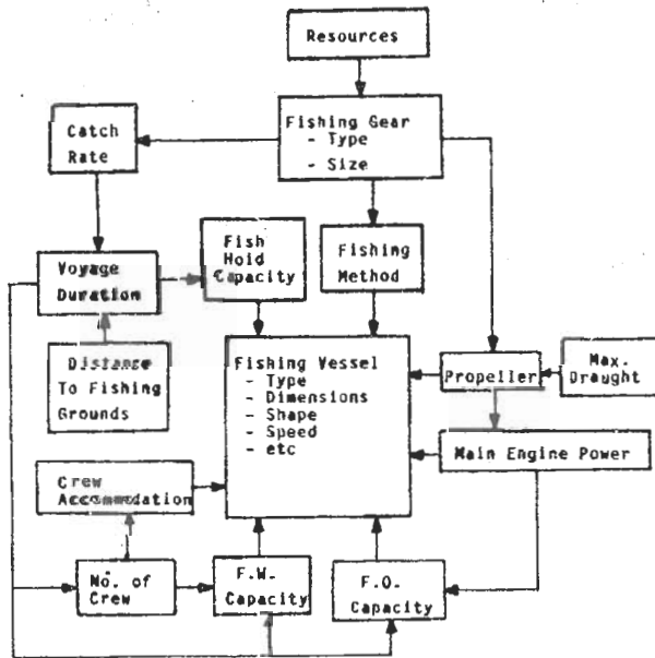
Figure 8. Fishing vessel design procedure.
