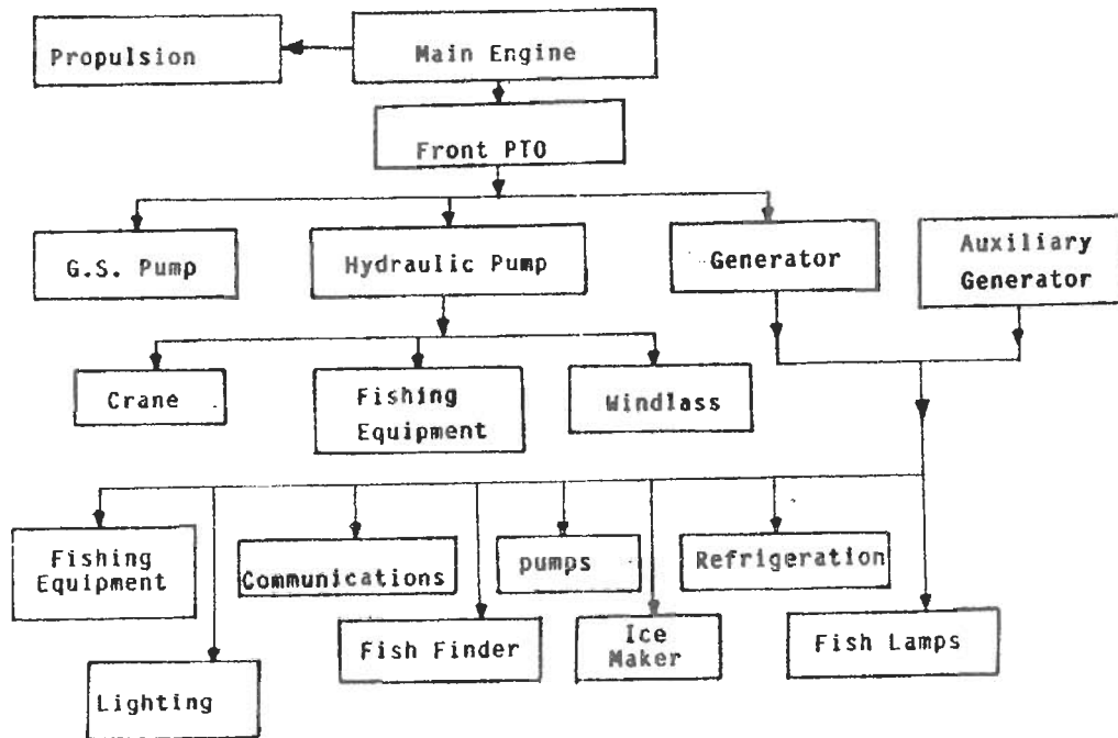
Figure 7. Fishing vessel power requirements.
