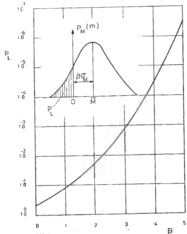
Figure 16. Relation between P_L and \beta .
