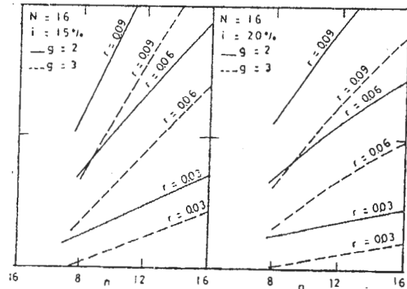
Figure 5-A. Variation of average annual cost of capital/ C_s with N, n, i, g, r .
